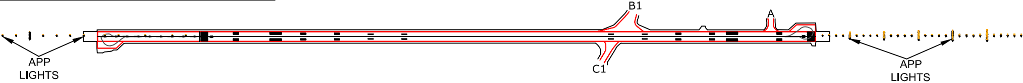
RWY 14/32 Marking Aids and exit way
