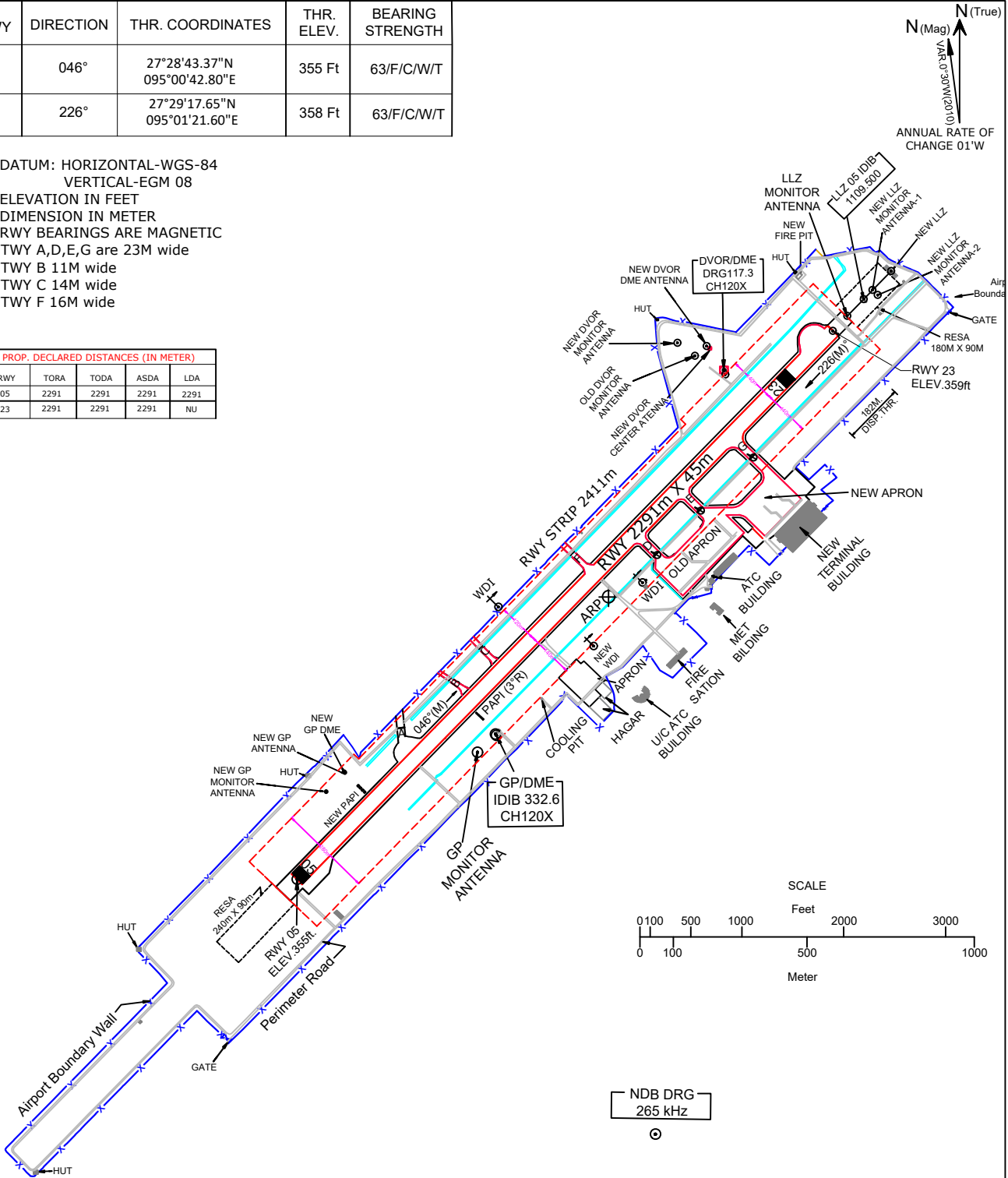
MARKING AIDS AND EXIT WAY RWY 05/23
